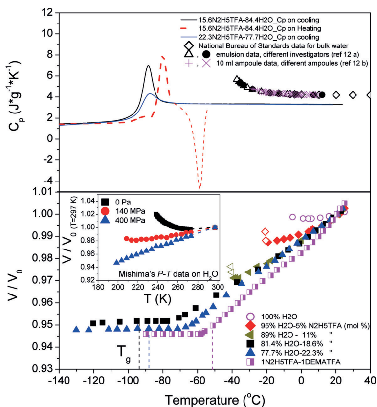
Figure 3. Upper panel: The C_p “spike” anomaly in two hydrazinium trifluoroacetate solutions during cooling, and also during subsequent heating for the more striking case. Comparison is made with the much-studied power law-diverging heat capacity of supercooled pure water. Lower panel: The volumes, relative to those at 25 °C, of 1) solutions of water + hydrazinium trifluoroacetate with water contents 100 to 77.7 mol % water. Onset of ice crystallization at high water contents shown by vertical jumps. Note, at lower water contents, the arrest of the solution volume well above the temperature of the heat capacity anomaly, and 2) an anhydrous binary ionic solution [DEMA + ][TFA - ] 0.5 [N 2 H 5 + ][TFA - ] 0.5 , with a simple glass transition arrest of volume. Vertical dashed lines indicate the values of the onset heating T_g for solutions of same color symbols. Inset: Behavior of the volume of supercooled water (from Ref. [15]) scaled to have common values at 297 K. Figure shows that the volume minimum disappears at about 140–160 MPa.
